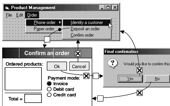
Figure 16: Derived presentation, dialog for 3 rd sub-task.
