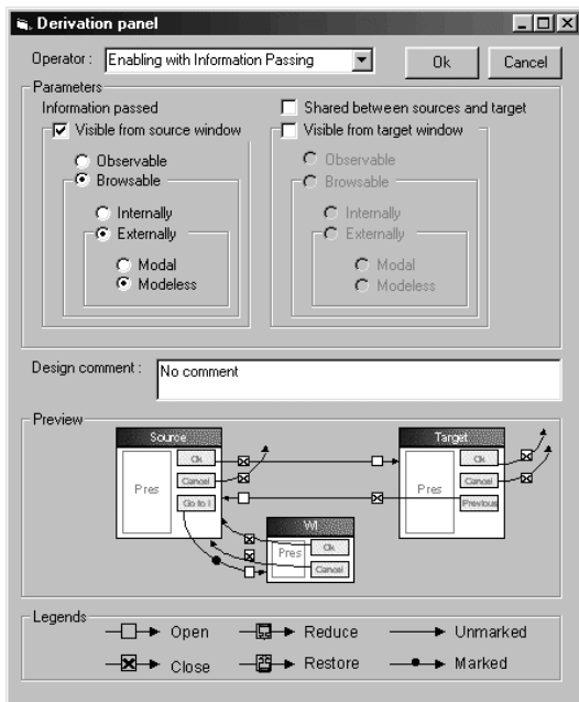
Figure 17: Guided definition of derivation rules.
