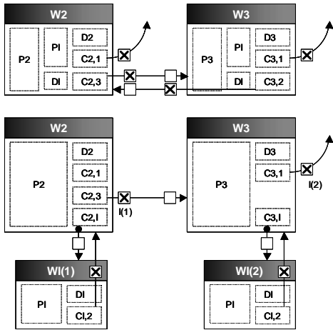
Figure 9: Changes when I is visible for T2 and T3 (a,b).
