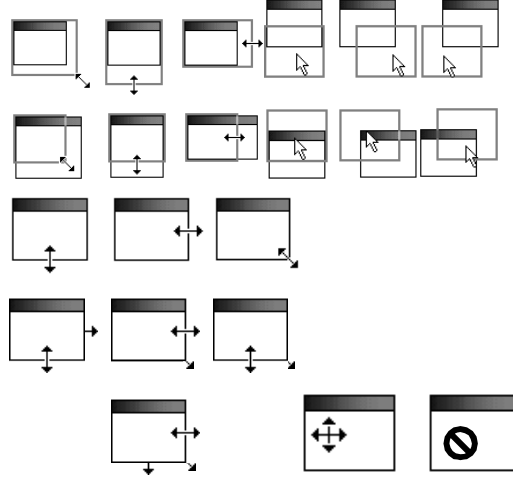
Figure 12: Allowed and prohibited window operations.
