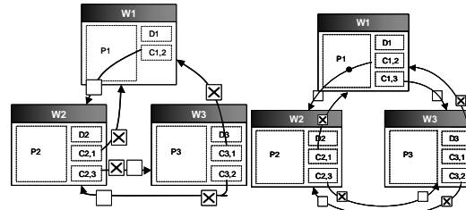
Figure 5. Alternative specifications for Enabling op.
