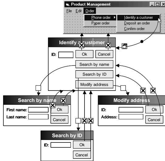
Figure 14: Derived presentation, dialog for 1 st sub-task.
