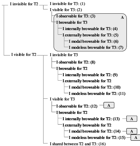
Figure 6: Decision tree of alternative specifications.
