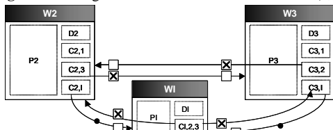
Figure 10: Change when I is shared.
