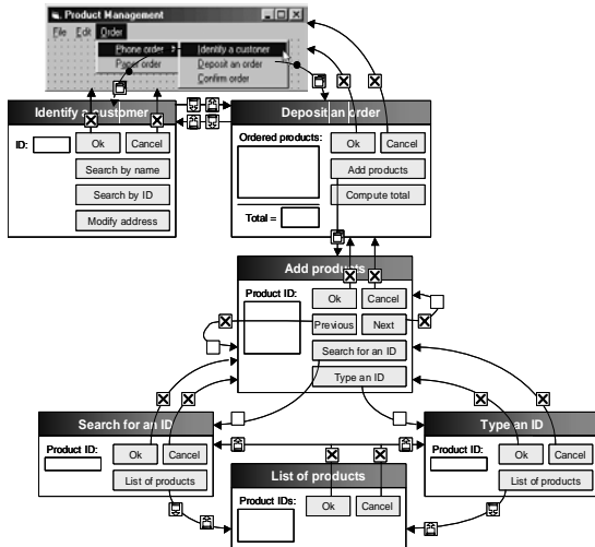
Fig. 15: Derived presentation, dialog for 2 nd sub-task.
