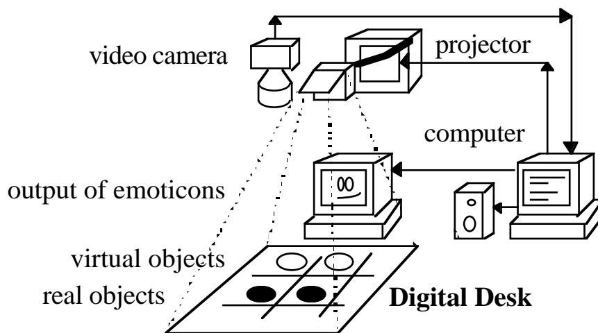
Figure 1: System architecture of the DigitalDesk.
