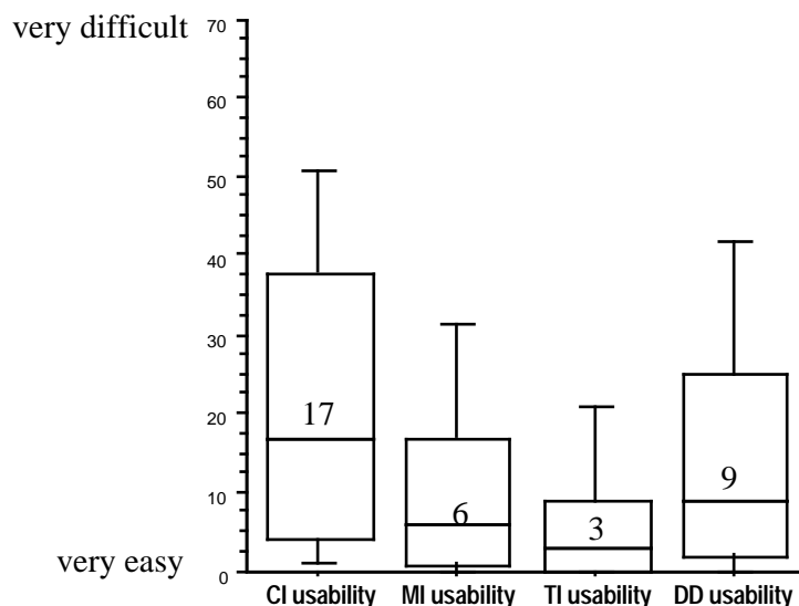
Figure 3: Box Plots of the four scales to estimate the "usability" of each interaction technique [the number inside the box is the median].
