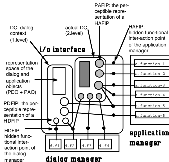
Figure 2. A schematic presentation of the I/O interface, the dialog and the application manager of an interactive system with a menu tree of two levels.
