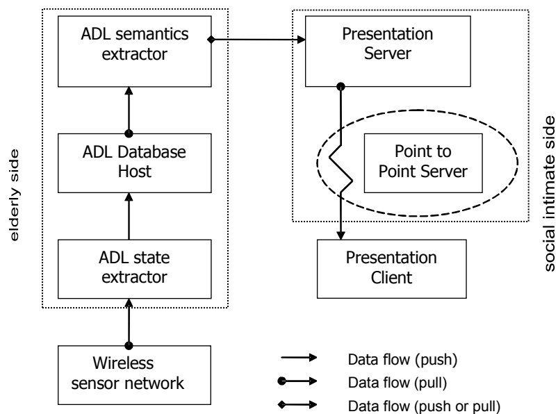
Figure 5. Overview of the prototype architecture, its components, and their location in the current experimental configuration.
